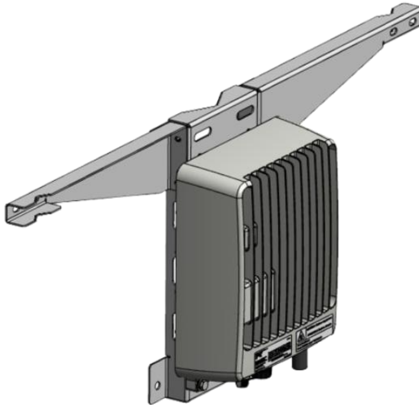
Figure 6: KONA Module with Mounting Bracket
