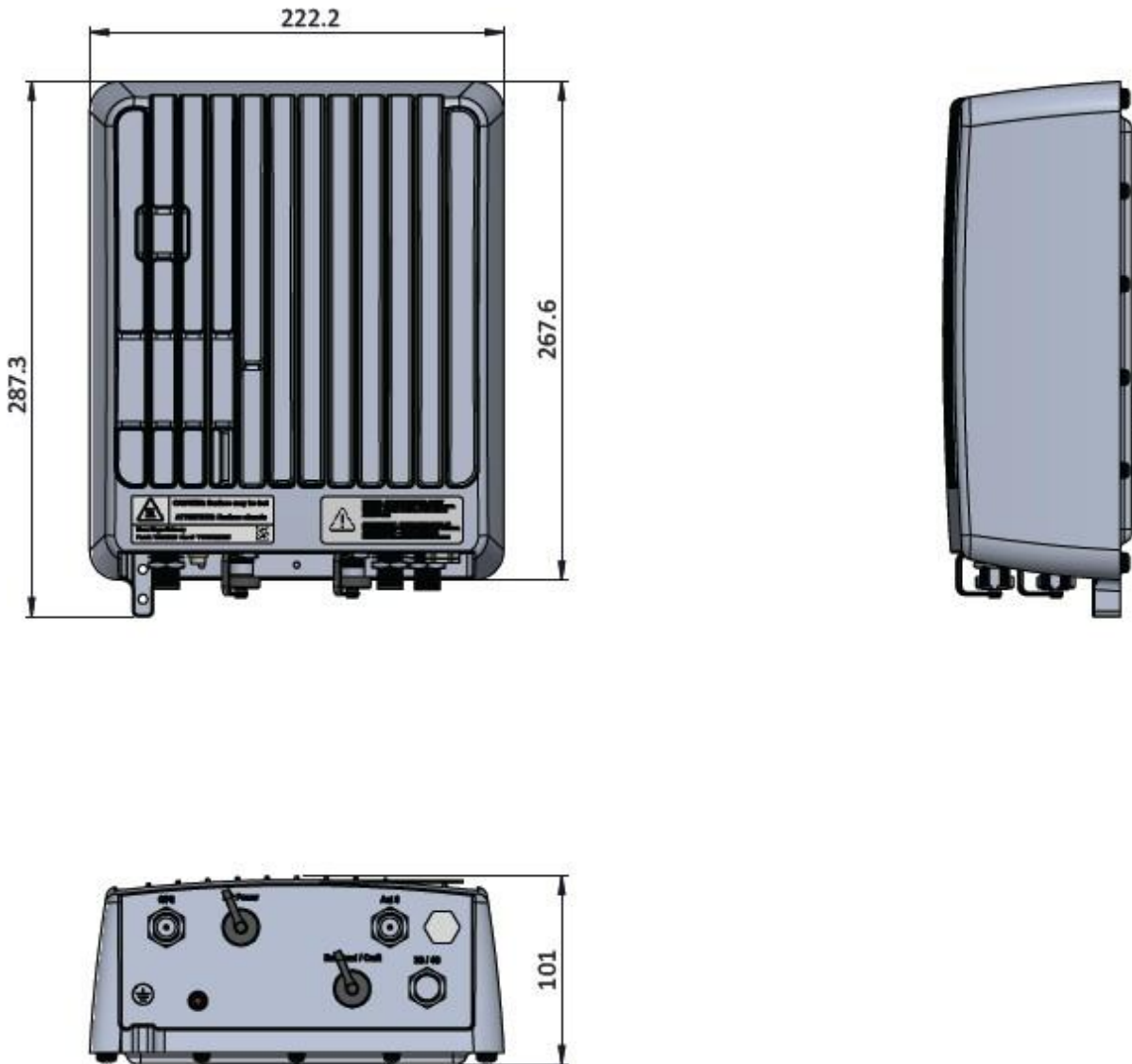
Figure 1: Kona HazLoc Mega Gateway
