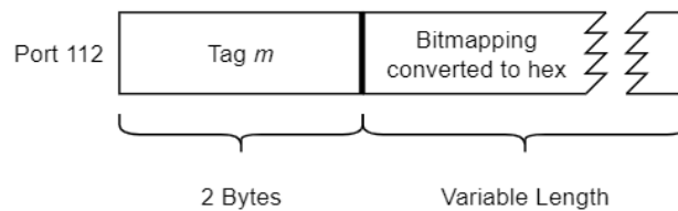
Figure 0-2: Bitmapping DL Format to Request Multiple Tagged Entries
