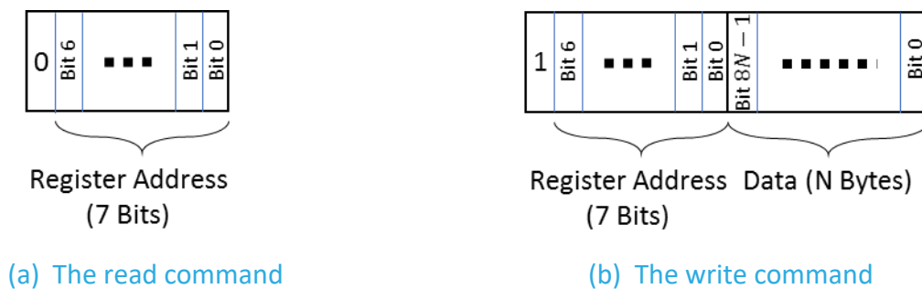
Figure 3-1: Format of a DL Configuration and Control Message Block
