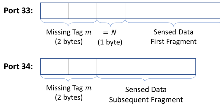
Figure 0-4: The Fragmented Data Forwarding Payload Format
