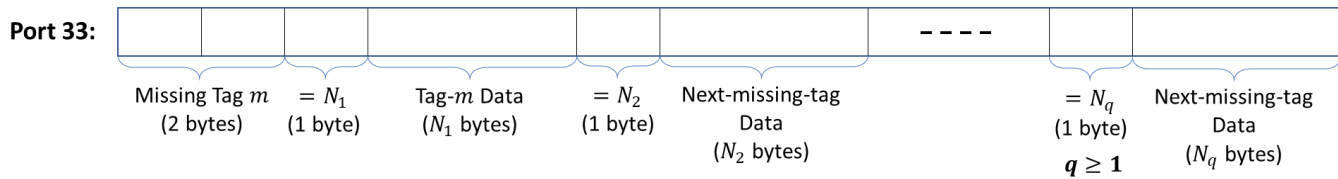
Figure 0-3: The Unfragmented Data Forwarding Payload Format
