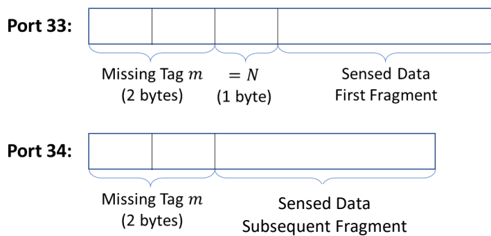
Figure 2-4: The Fragmented Data Forwarding Payload Format
