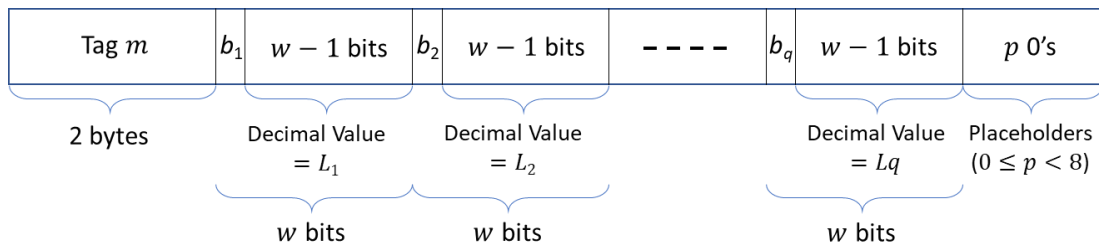
Figure 0-3: RLE Packet format for Requesting Multiple Tag Entries
