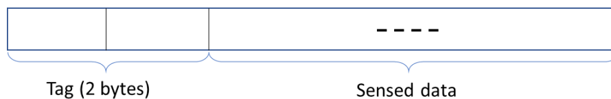
Figure 1-8: Tagged LoRaWAN Frame Payload
