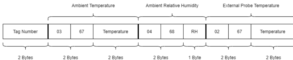
Figure 2-2: The Tagged UL Frame Payload Format
