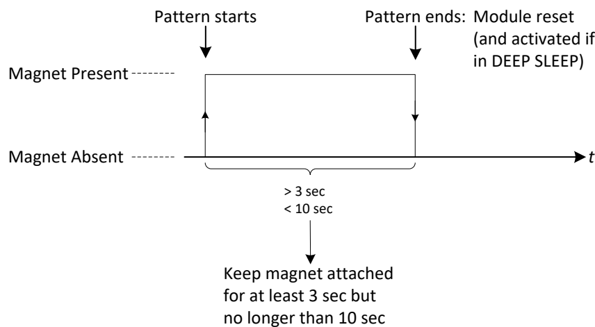
Figure 1-5: The Magnetic Reset/Wake-Up Pattern
