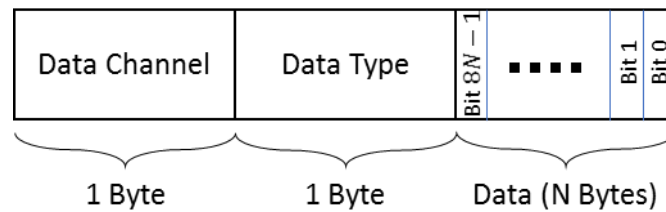
Figure 2-1: The UL Frame Payload Format for Non-Tagged Transducer Data
