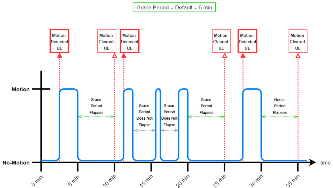
Figure 1-7: Example Sequence of Accelerometer Events and UL Reports
