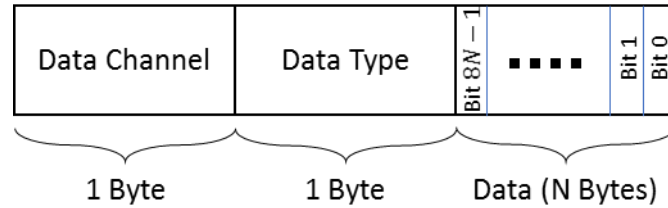
Figure 0-1: The UL Frame Payload Format for Non-Tagged Transducer Data
