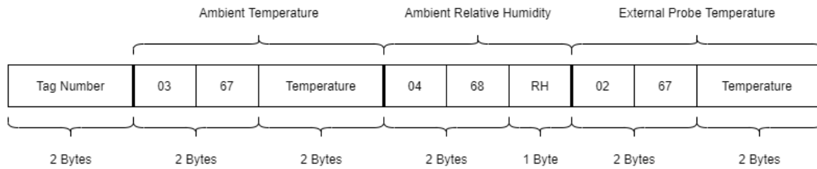
Figure 0-2: The Tagged UL Frame Payload Format
