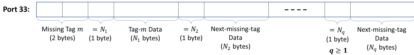
Figure 2-3: The Unfragmented Data Forwarding Payload Format
