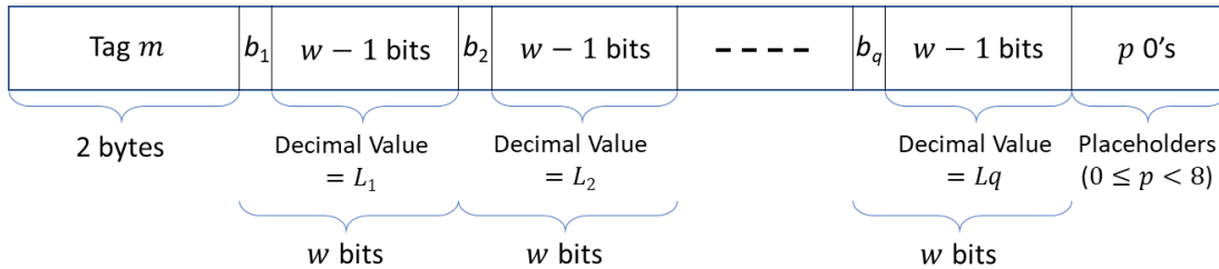
Figure 3-4: RLE Packet format for Requesting Multiple Tag Entries
